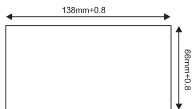
Panel Cutout
