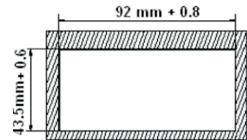
Installation Cutout
